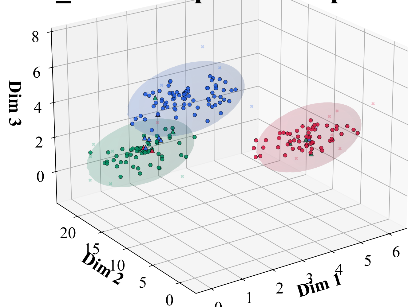
S_encoder Space — Explore (z=0)
